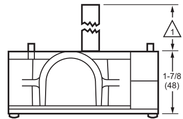
Fig. 17. Q5020 Actuator Linkage dimensions in in. (mm).
